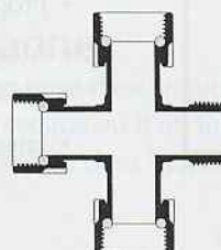
Croix union 1" M x 1" F x 1" F x 1" F
